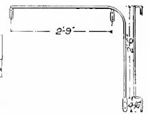
Figs. 1255-1256. Platform Hand-rail (4).
